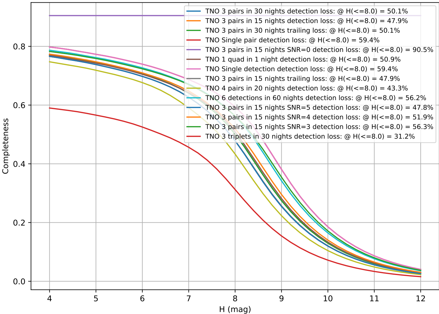
weather_cloudso20v3.5_10yrs: CumulativeCompleteness
