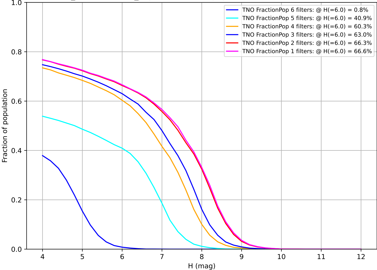
weather_cloudso20v3.5_10yrs: Fraction of population with colors in X filters TNO
