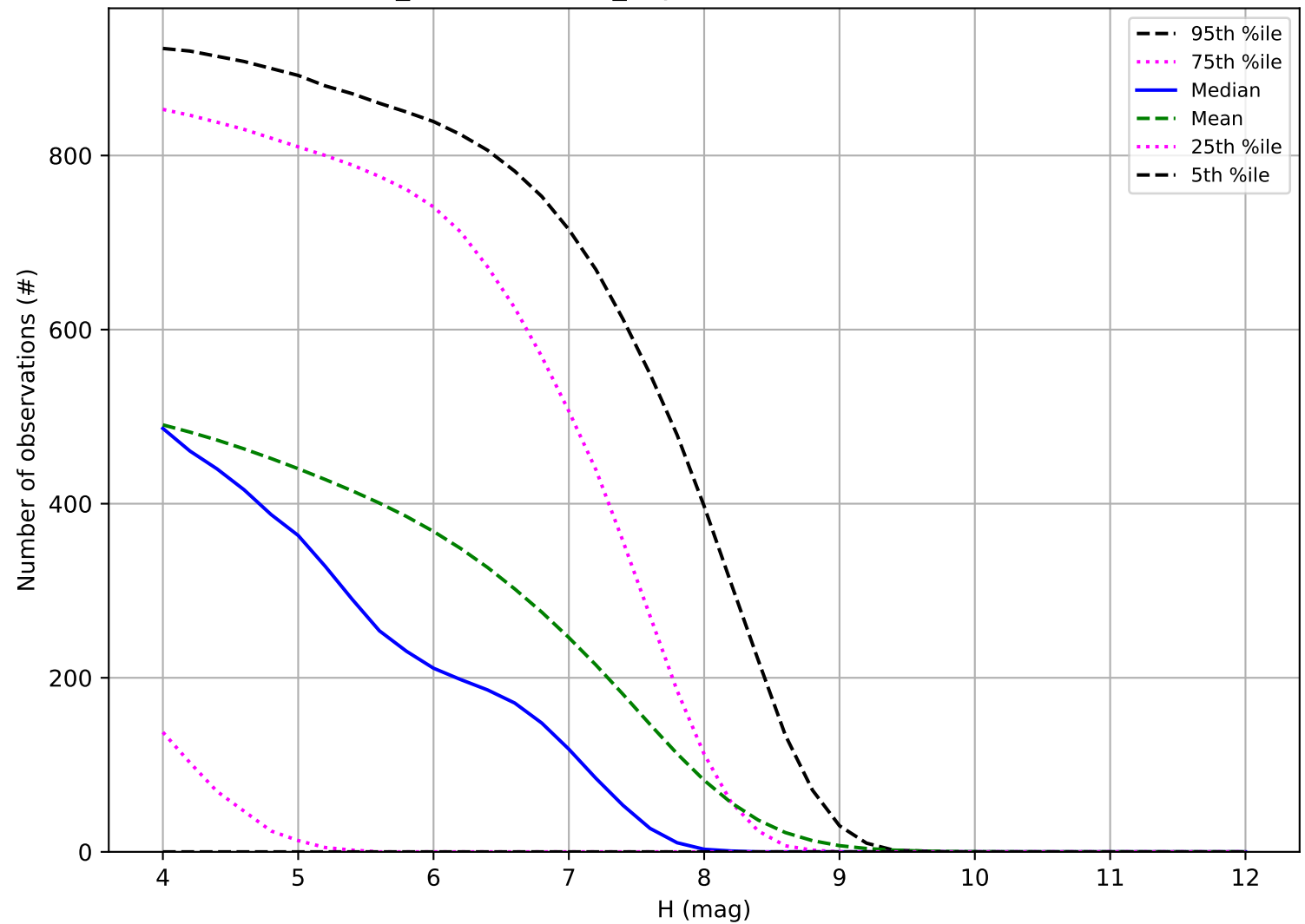
weather_cloudso20v3.5_10yrs: Number of observations TNO
