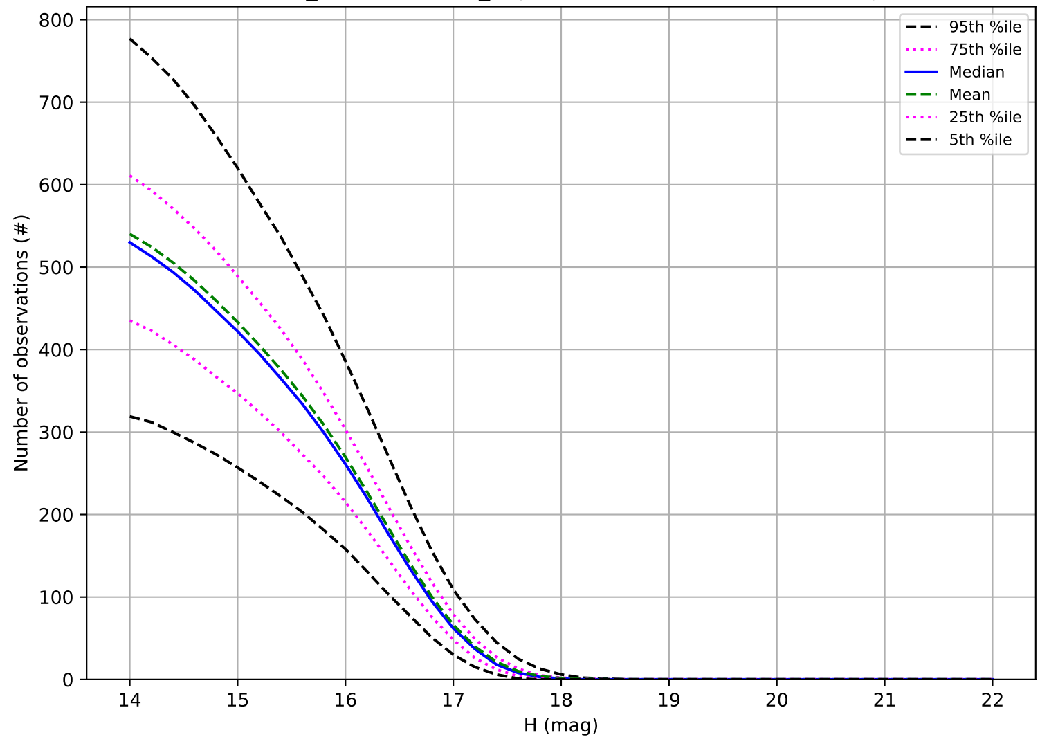
weather_cloudso20v3.5_10yrs: Number of observations Trojan
