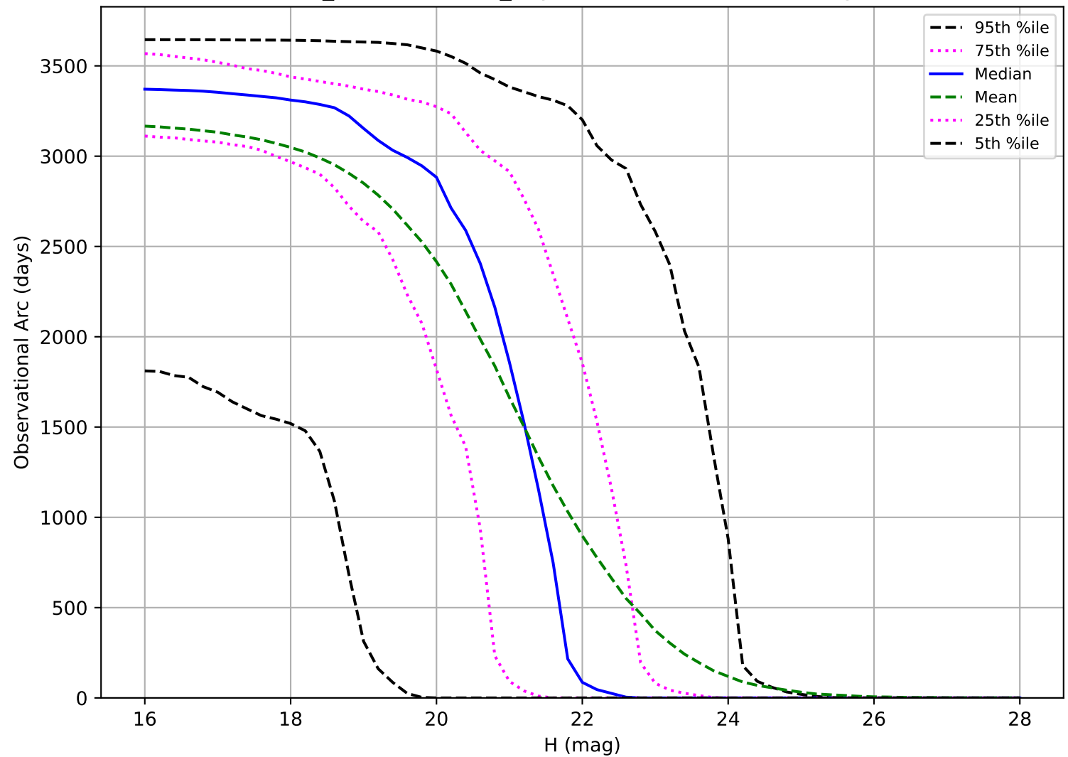
weather_cloudso20v3.5_10yrs: Observational Arc Length NEO
