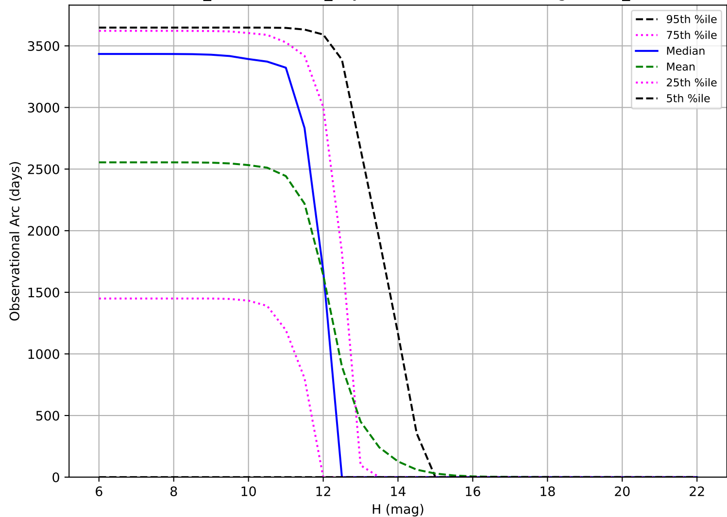
weather_cloudso20v3.5_10yrs: Observational Arc Length OCC_r20
