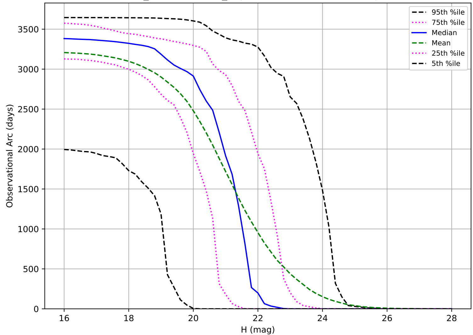
weather_cloudso20v3.5_10yrs: Observational Arc Length PHA
