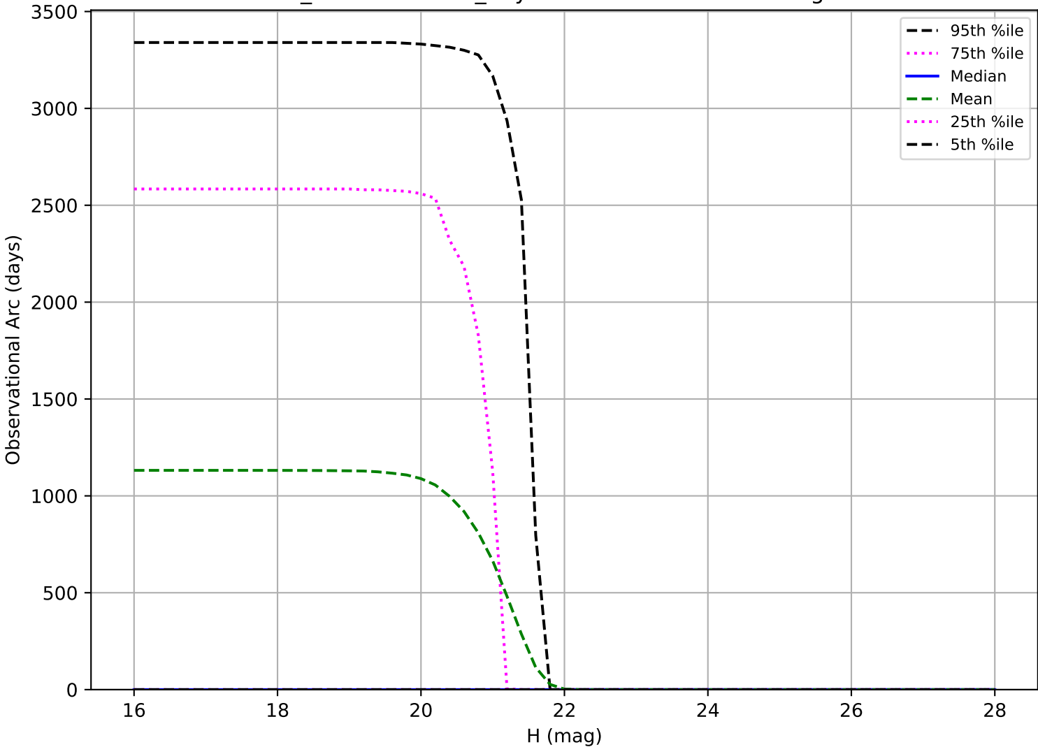
weather_cloudso20v3.5_10yrs: Observational Arc Length Vatra
