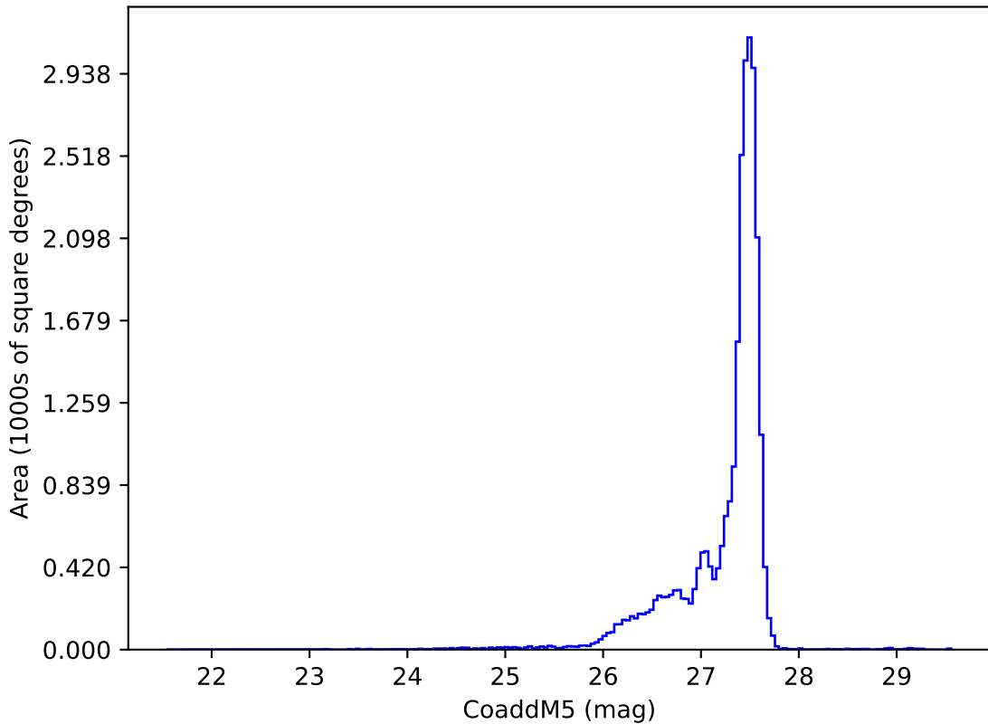
weather_cloudso2v3.5_10yrs : CoaddM5
