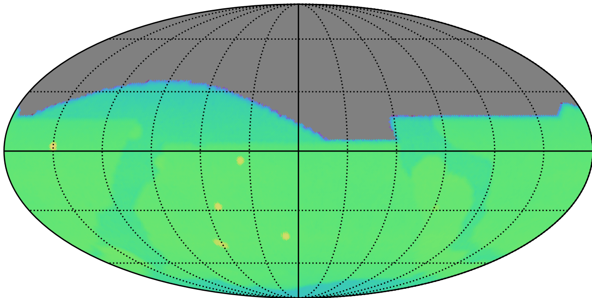
weather_cloudso2v3.5_10yrs : CoaddM5
