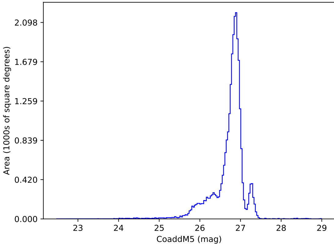
weather_cloudso2v3.5_10yrs g: CoaddM5
