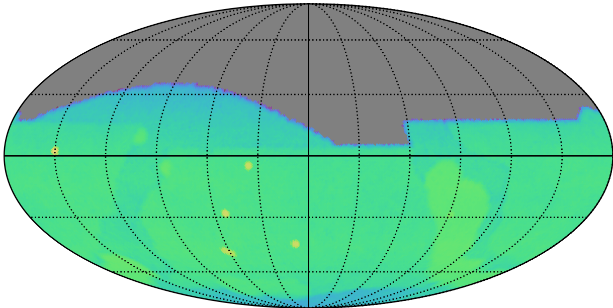
weather_cloudso2v3.5_10yrs g: CoaddM5
