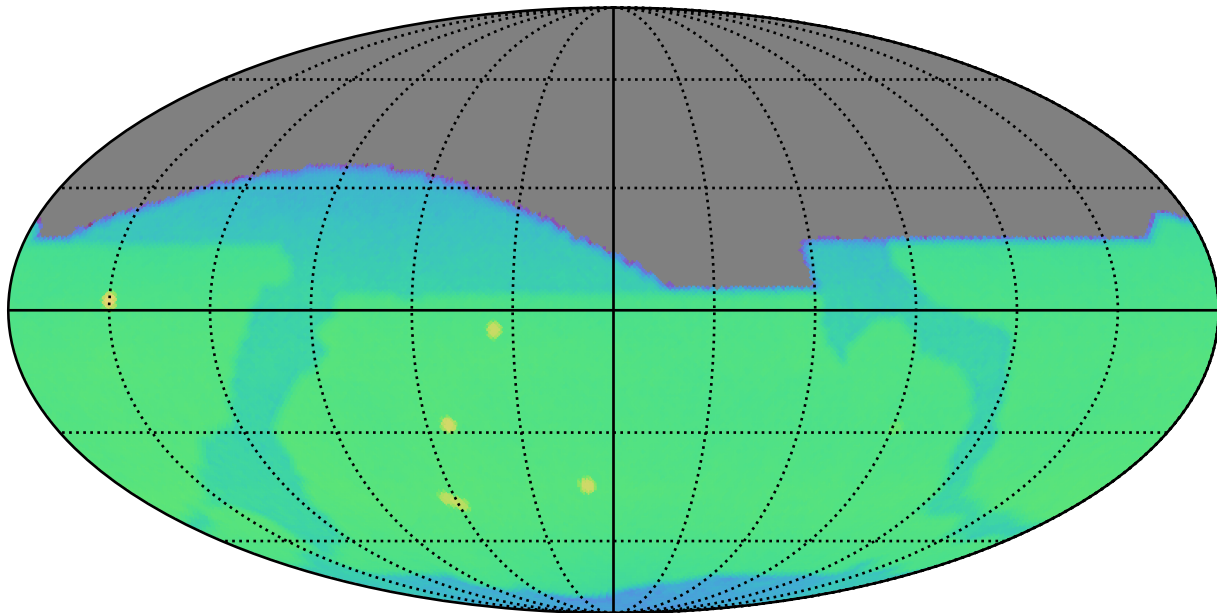
weather_cloudso2v3.5_10yrs r: CoaddM5
