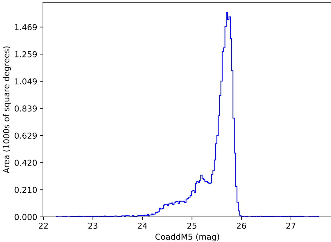
weather_cloudso2v3.5_10yrs u: CoaddM5
