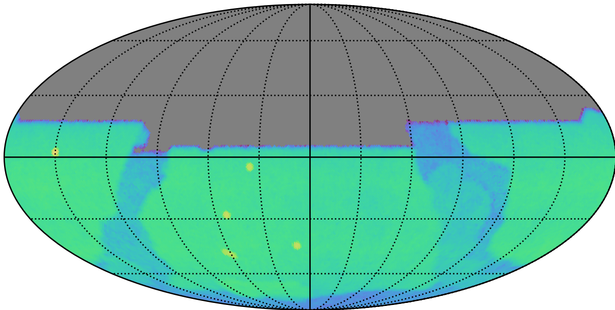
weather_cloudso2v3.5_10yrs u: CoaddM5
