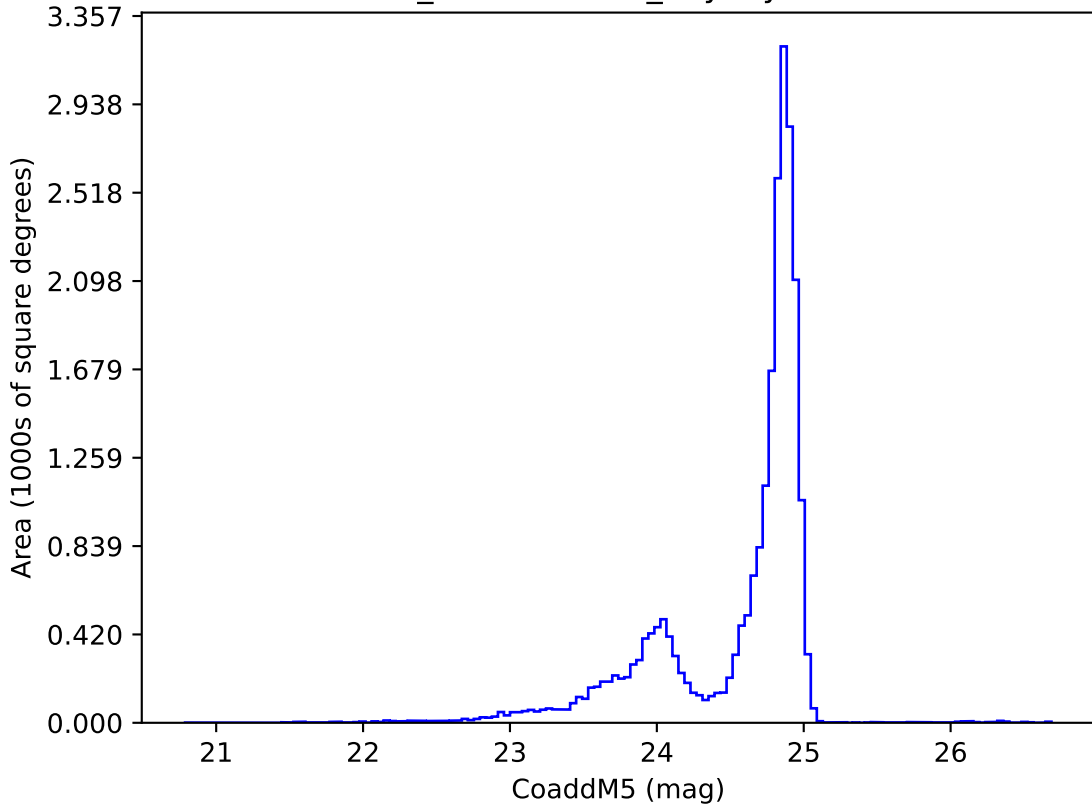
weather_cloudso2v3.5_10yrs y: CoaddM5
