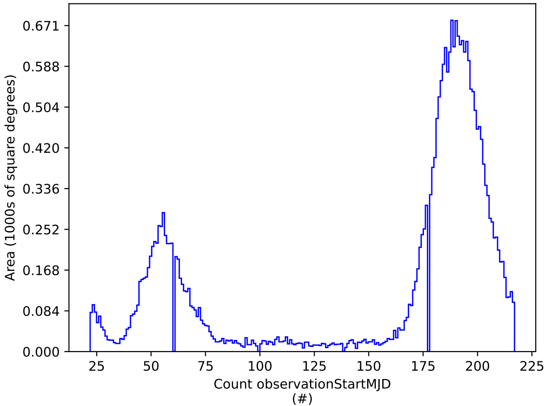
weather_cloudso2v3.5_10yrs i: Count observationStartMJD
