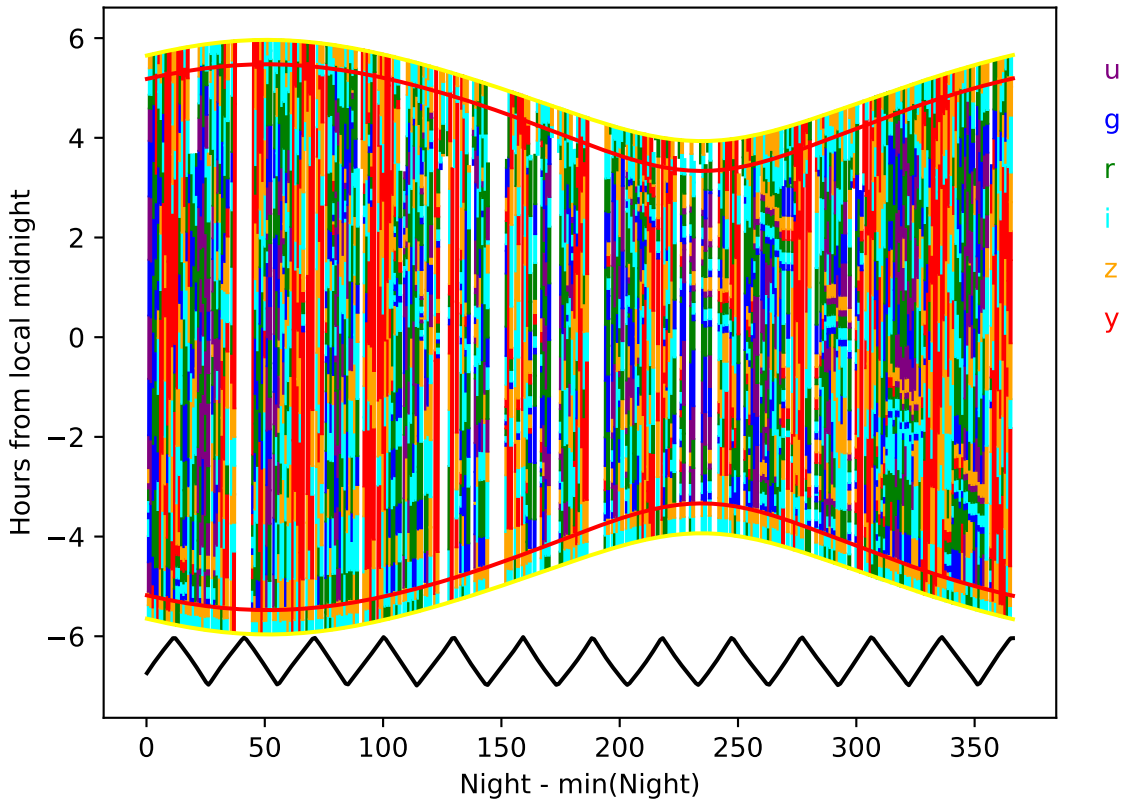
weather_cloudso2v3.5_10yrs year 0-1: Hourglass
