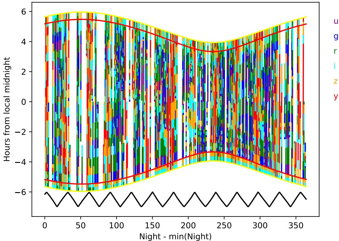
weather_cloudso2v3.5_10yrs year 9-10: Hourglass
