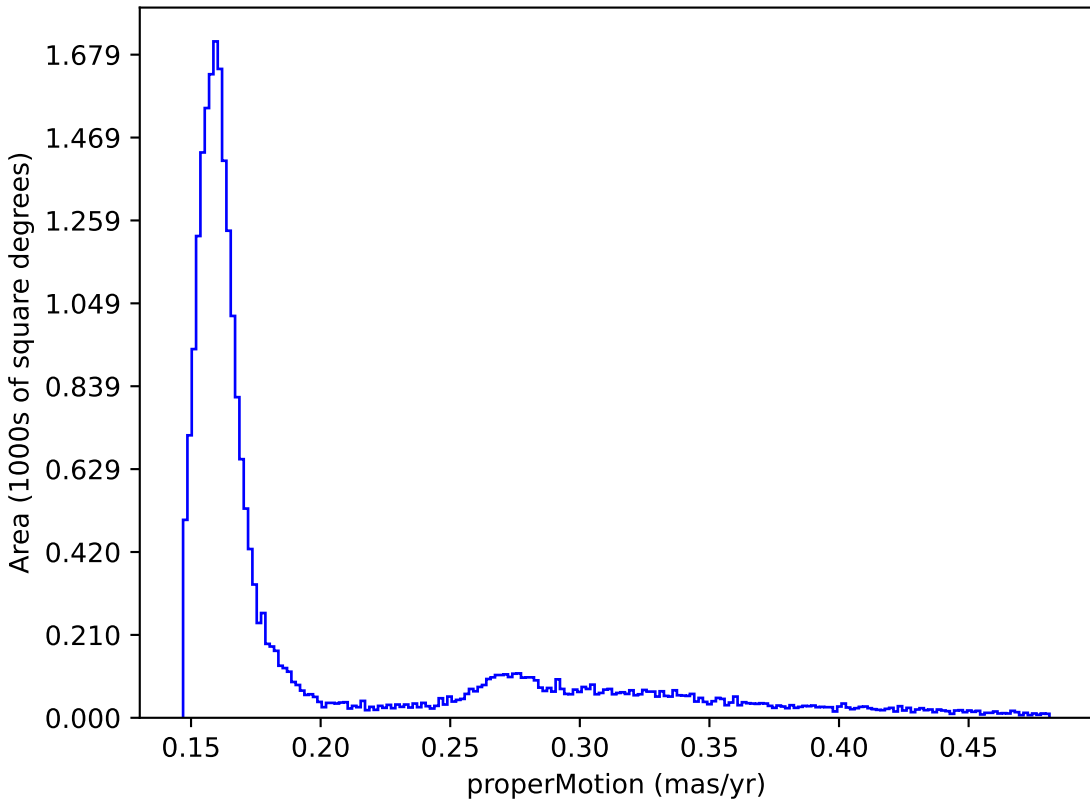
weather_cloudso2v3.5_10yrs : properMotion
