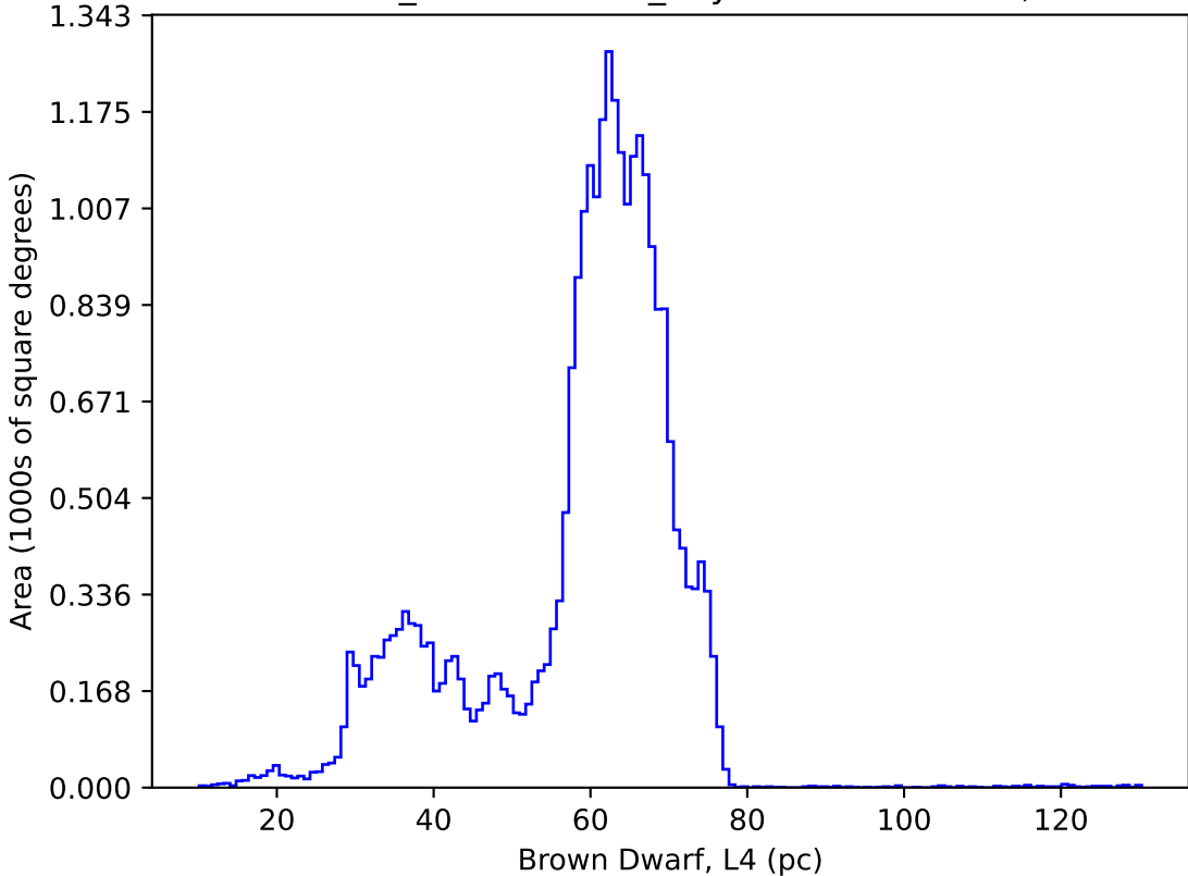
weather_cloudso2v3.5_10yrs : Brown Dwarf, L4
