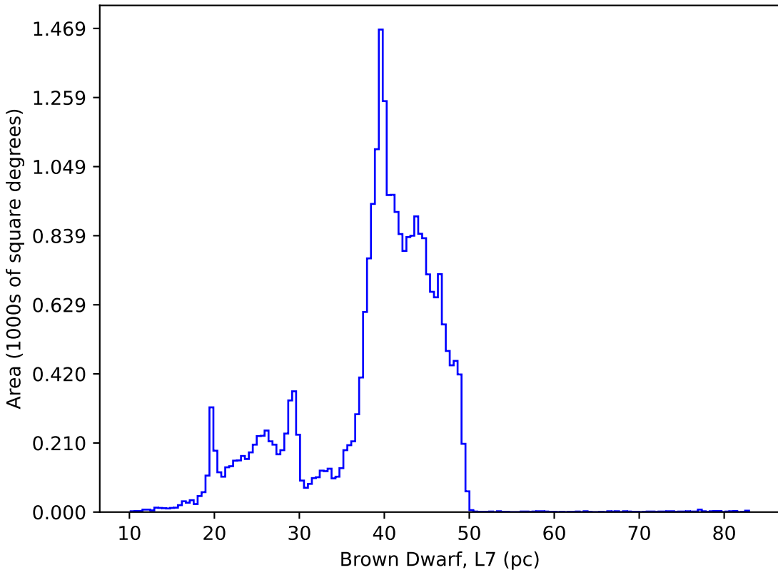
weather_cloudso2v3.5_10yrs : Brown Dwarf, L7
