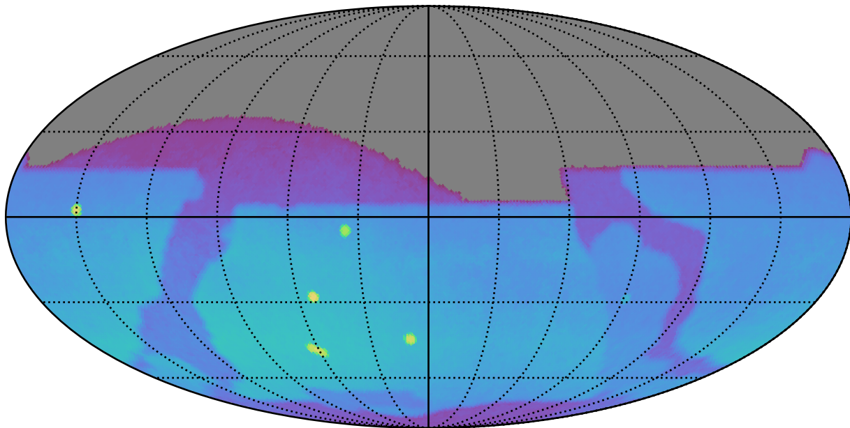
weather_cloudso2v3.5_10yrs : Brown Dwarf, L7
