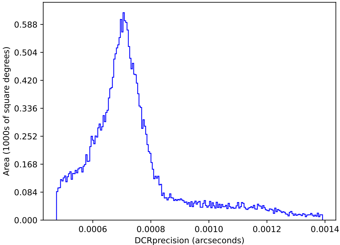
weather_cloudso2v3.5_10yrs : DCRprecision
