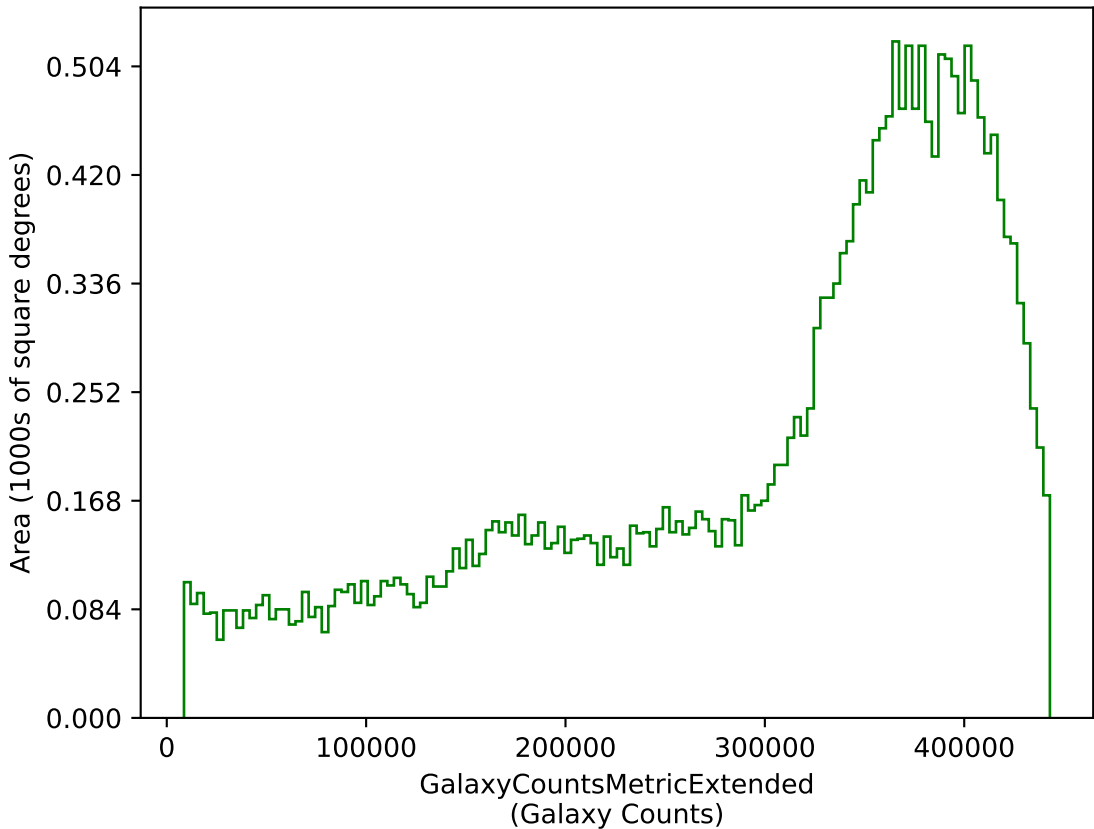
weather_cloudso2v3.5_10yrs g: GalaxyCountsMetricExtended
