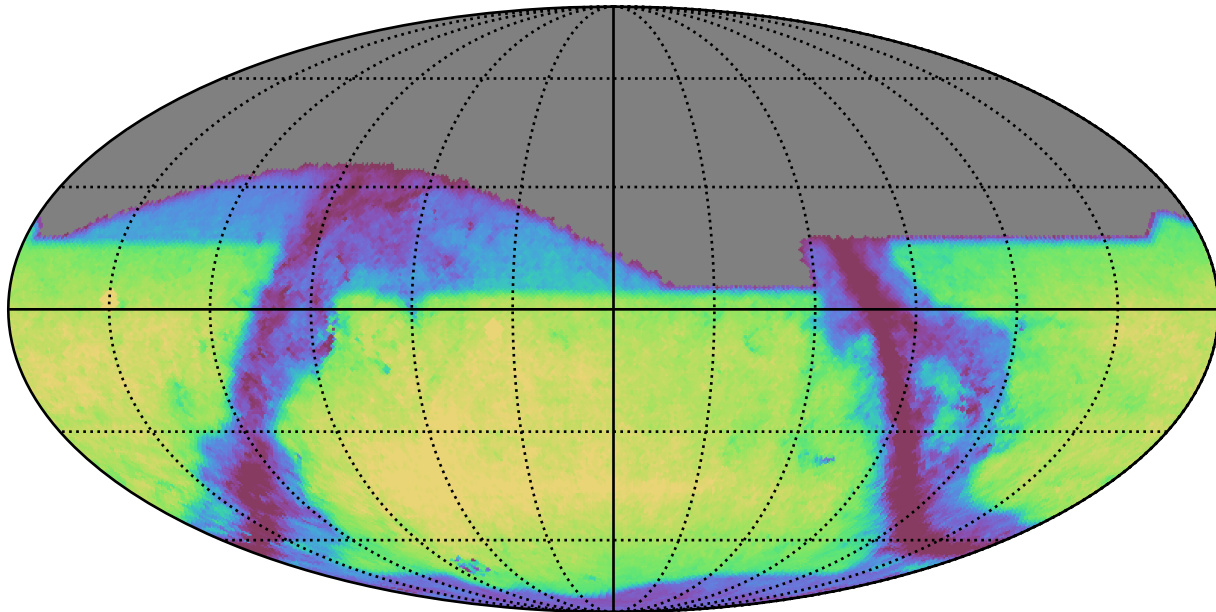
weather_cloudso2v3.5_10yrs i: GalaxyCountsMetricExtended
