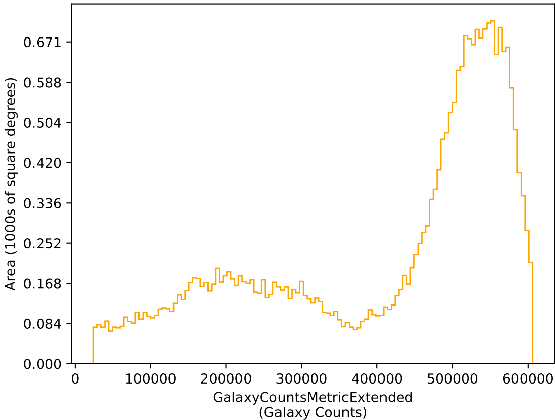
weather_cloudso2v3.5_10yrs r: GalaxyCountsMetricExtended
