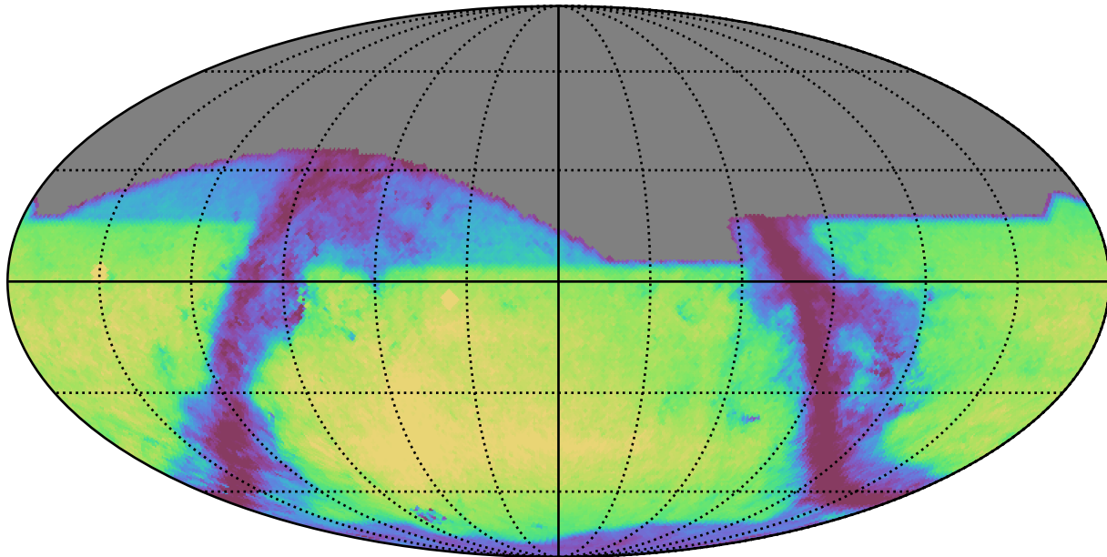
weather_cloudso2v3.5_10yrs r: GalaxyCountsMetricExtended
