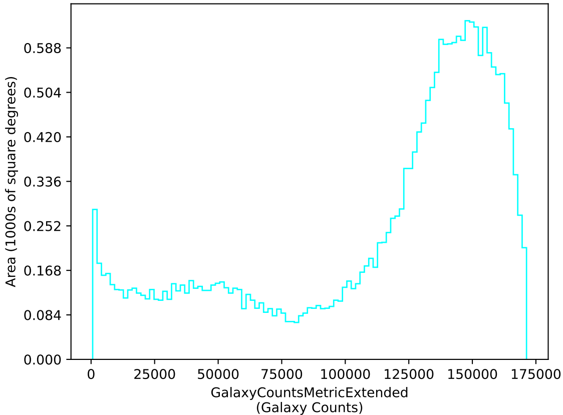
weather_cloudso2v3.5_10yrs u: GalaxyCountsMetricExtended
