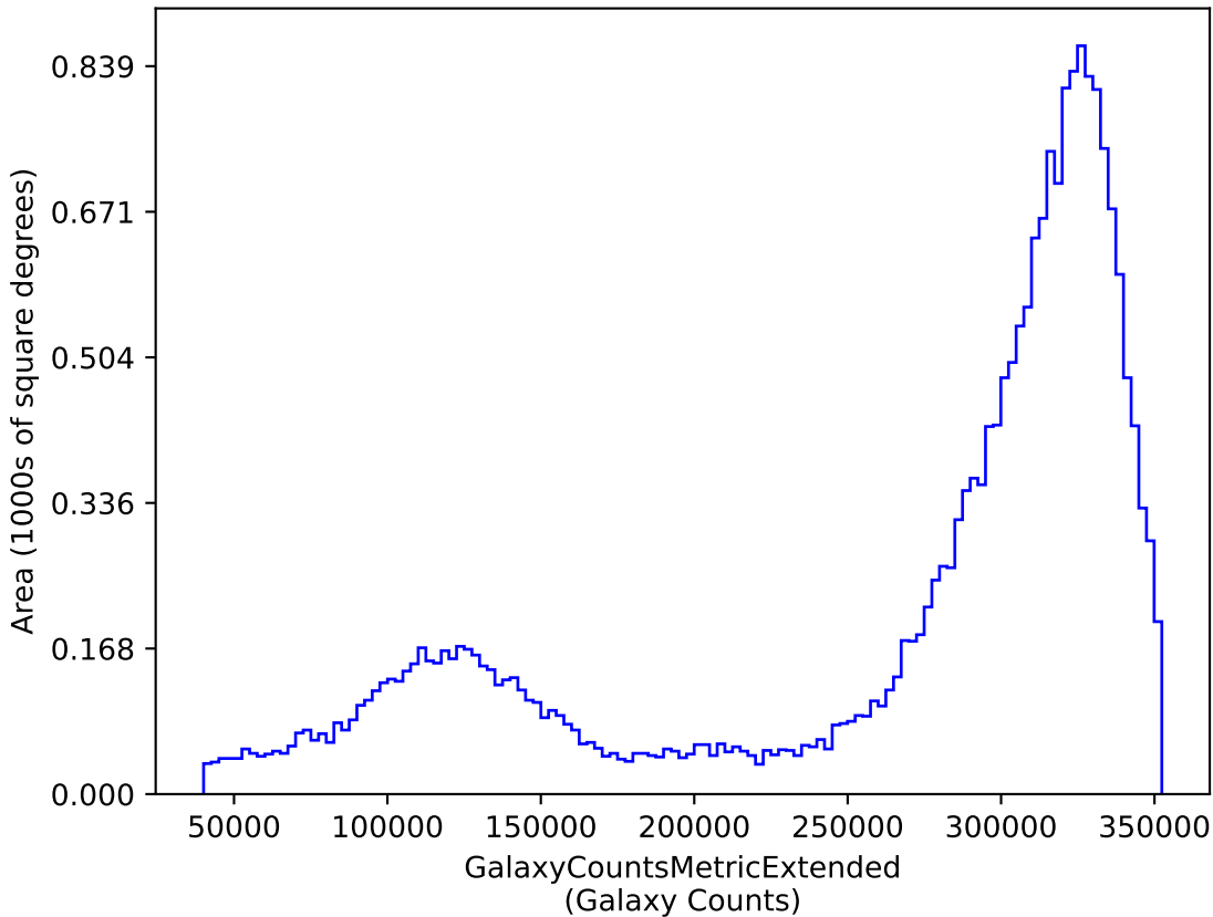
weather_cloudso2v3.5_10yrs y: GalaxyCountsMetricExtended
