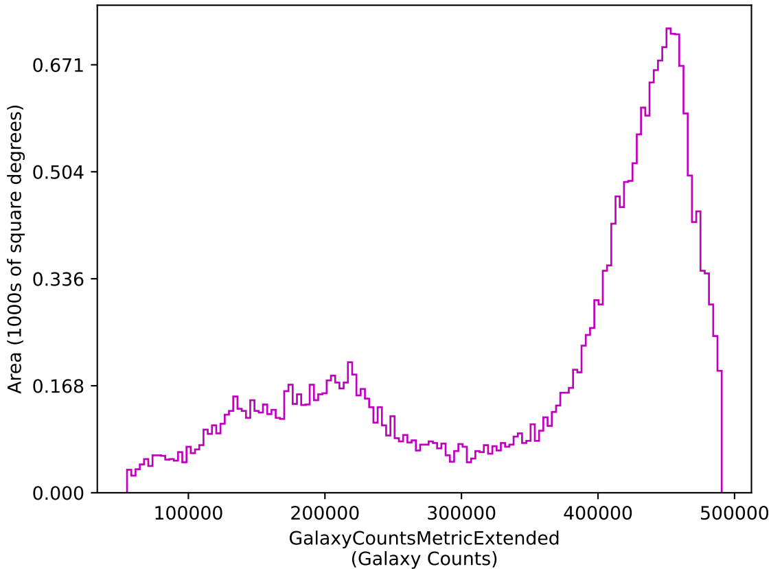
weather_cloudso2v3.5_10yrs z: GalaxyCountsMetricExtended
