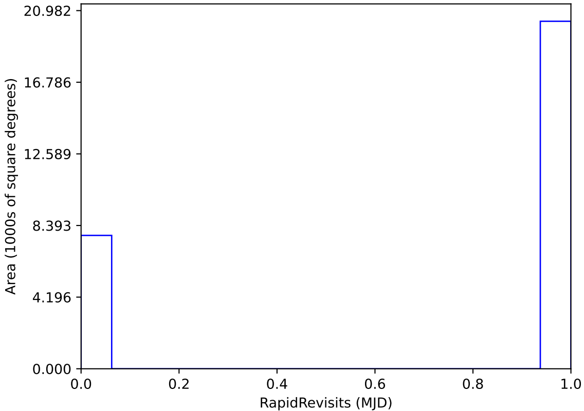
weather_cloudso2v3.5_10yrs : RapidRevisits
