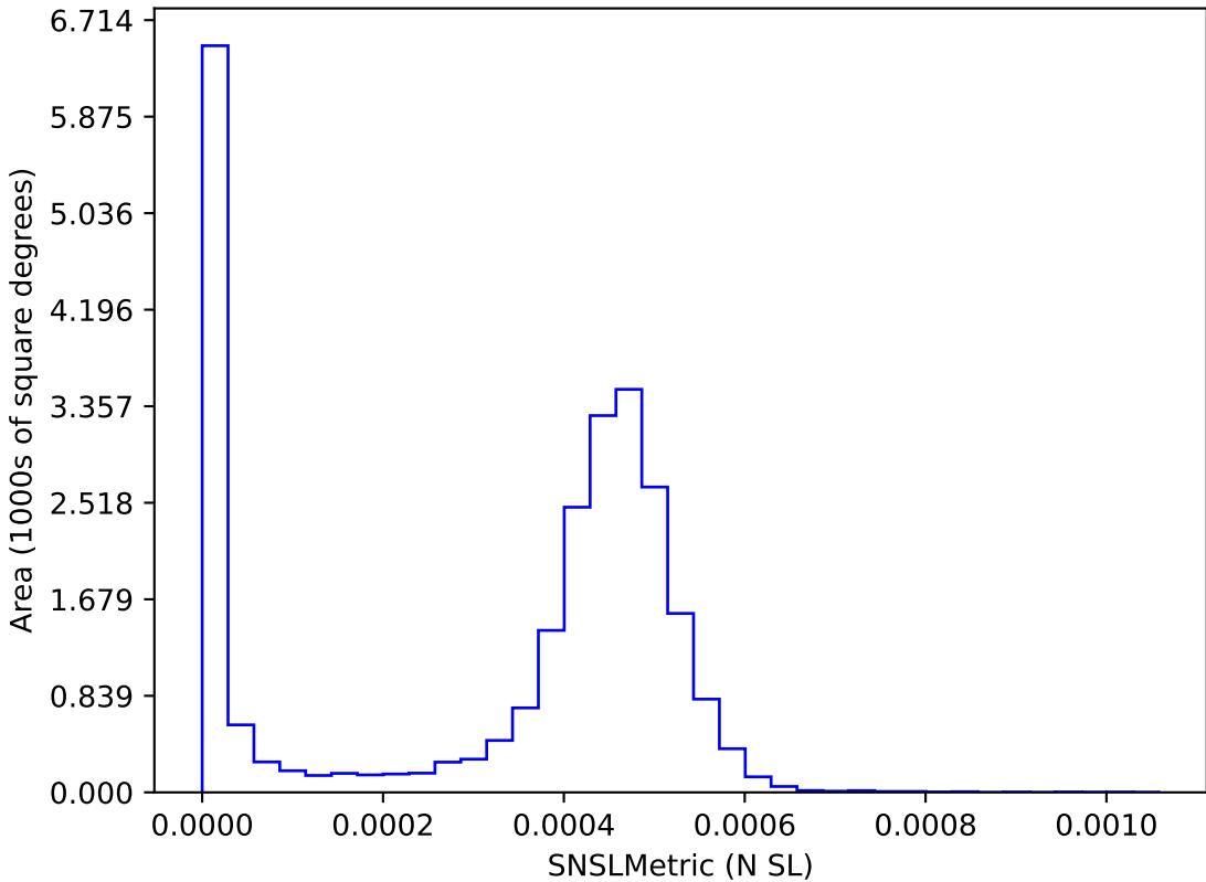
weather_cloudso2v3.5_10yrs : SNSLMetric
