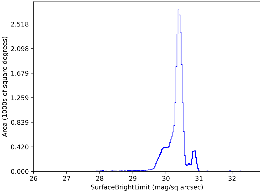
weather_cloudso2v3.5_10yrs g: SurfaceBrightLimit
