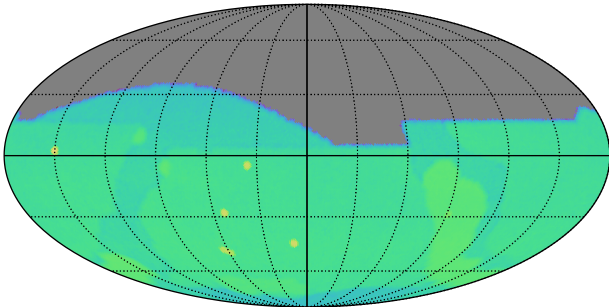
weather_cloudso2v3.5_10yrs g: SurfaceBrightLimit
