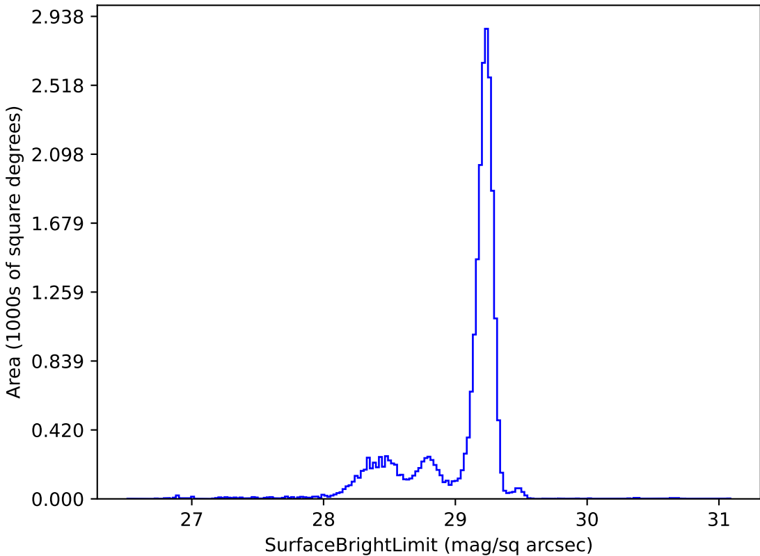
weather_cloudso2v3.5_10yrs u: SurfaceBrightLimit
