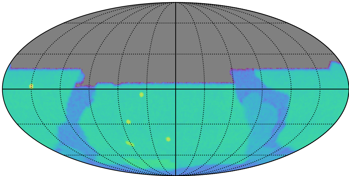
weather_cloudso2v3.5_10yrs u: SurfaceBrightLimit
