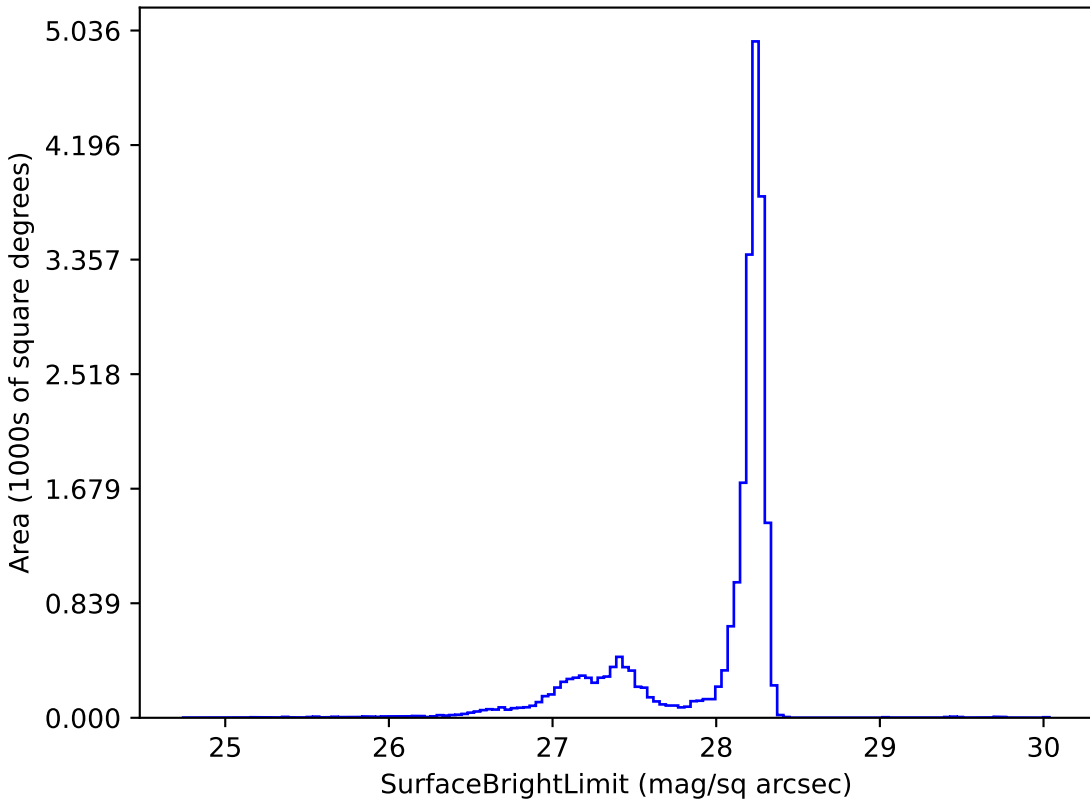
weather_cloudso2v3.5_10yrs y: SurfaceBrightLimit
