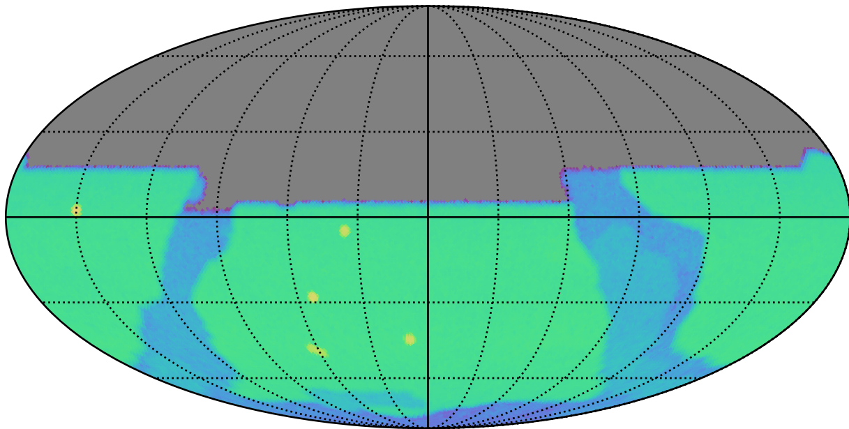
weather_cloudso2v3.5_10yrs y: SurfaceBrightLimit
