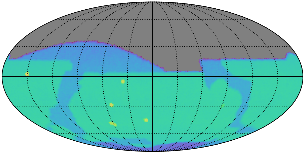
weather_cloudso2v3.5_10yrs z: SurfaceBrightLimit
