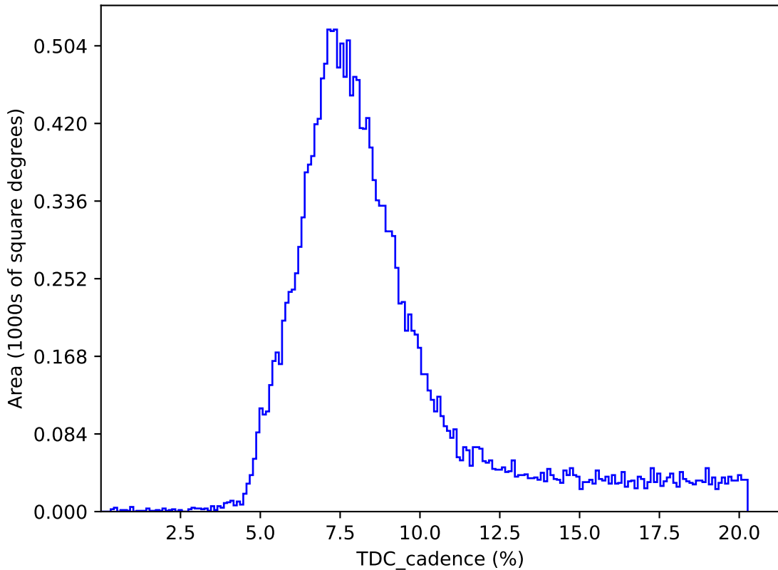
weather_cloudso2v3.5_10yrs : TDC_cadence
