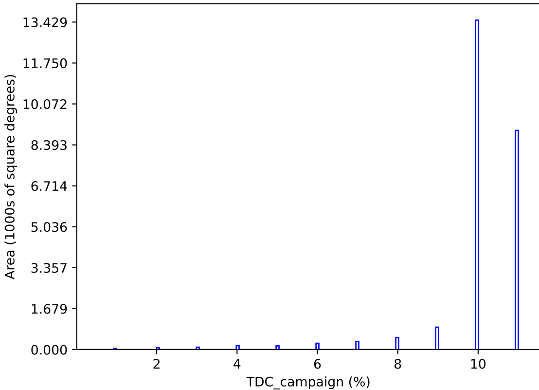
weather_cloudso2v3.5_10yrs : TDC_campaign
