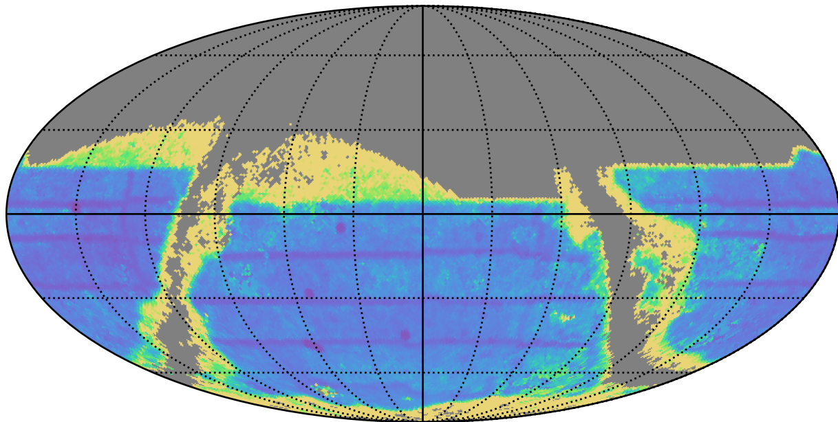
weather_cloudso2v3.5_10yrs : TDC_precision
