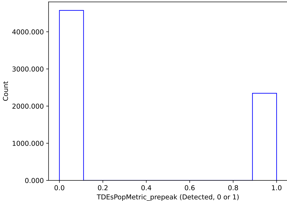
weather_cloudso2v3.5_10yrs : TDEsPopMetric_prepeak
