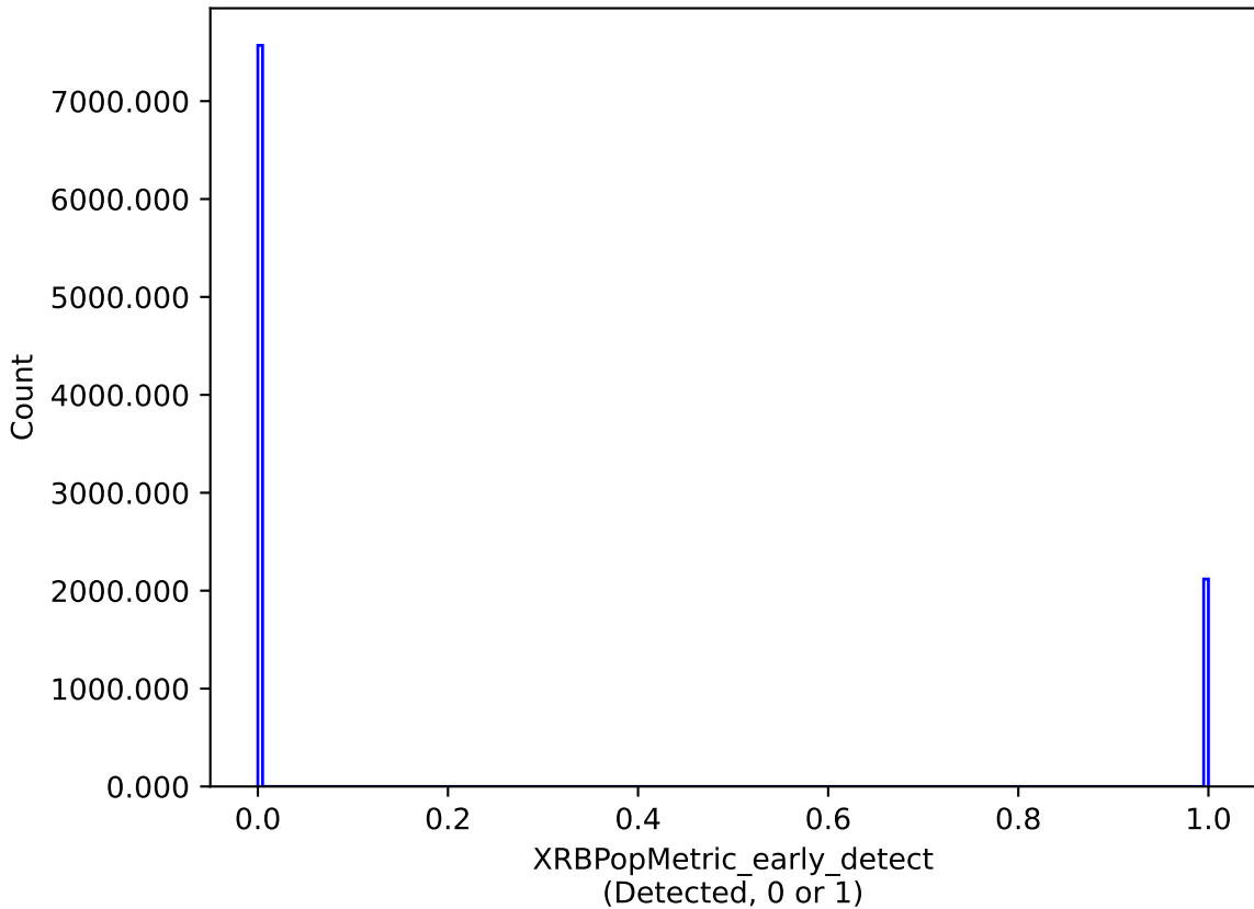
weather_cloudso2v3.5_10yrs : XRBPoMetric_early_detect
