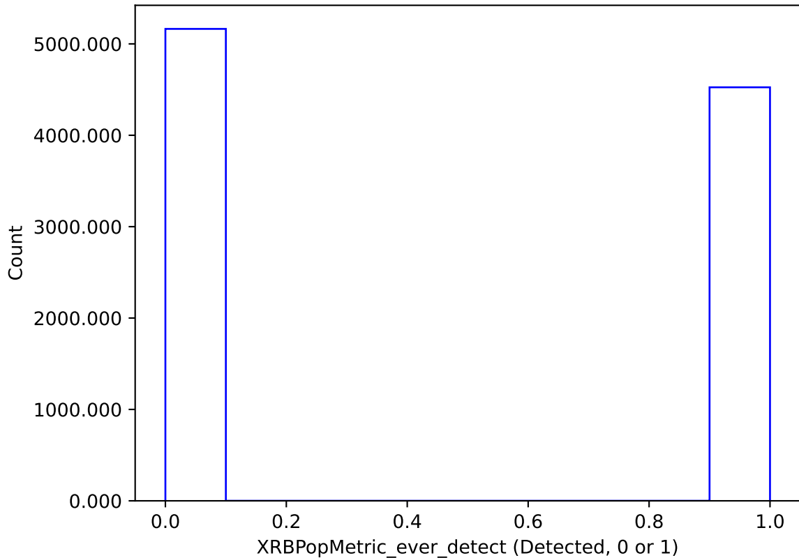
weather_cloudso2v3.5_10yrs : XRBPoMetric_ever_detect
