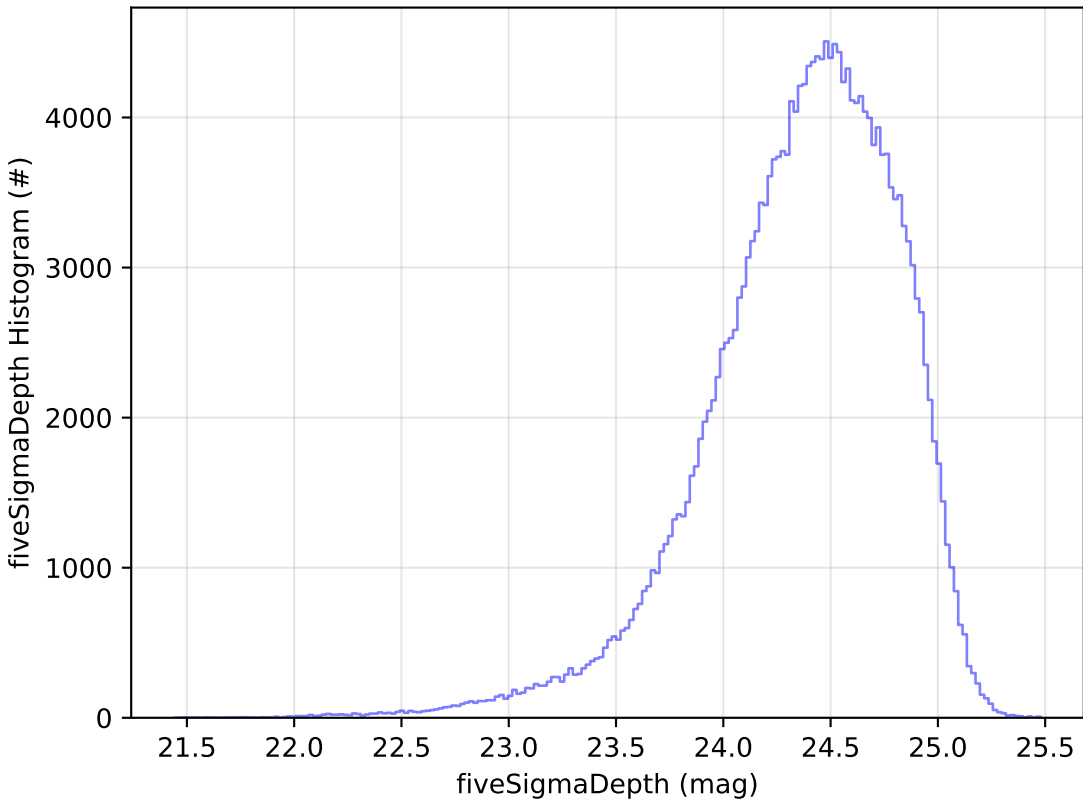
weather_cloudso2v3.5_10yrs g: fiveSigmaDepth Histogram
