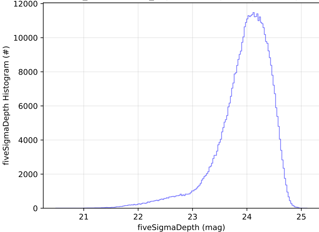
weather_cloudso2v3.5_10yrs r: fiveSigmaDepth Histogram
