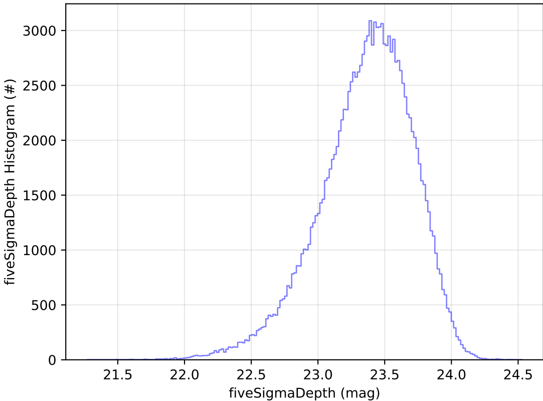
weather_cloudso2v3.5_10yrs u: fiveSigmaDepth Histogram
