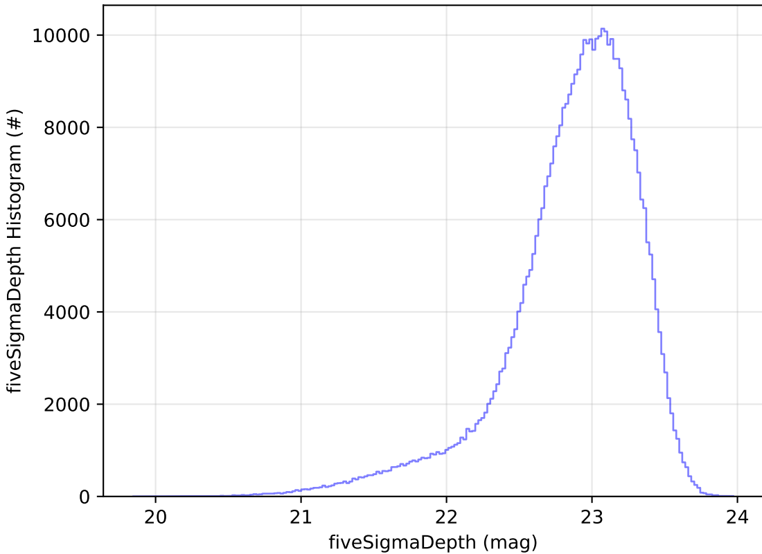
weather_cloudso2v3.5_10yrs z: fiveSigmaDepth Histogram
